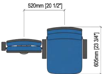
Abatible Foldable Seat Frontwards
